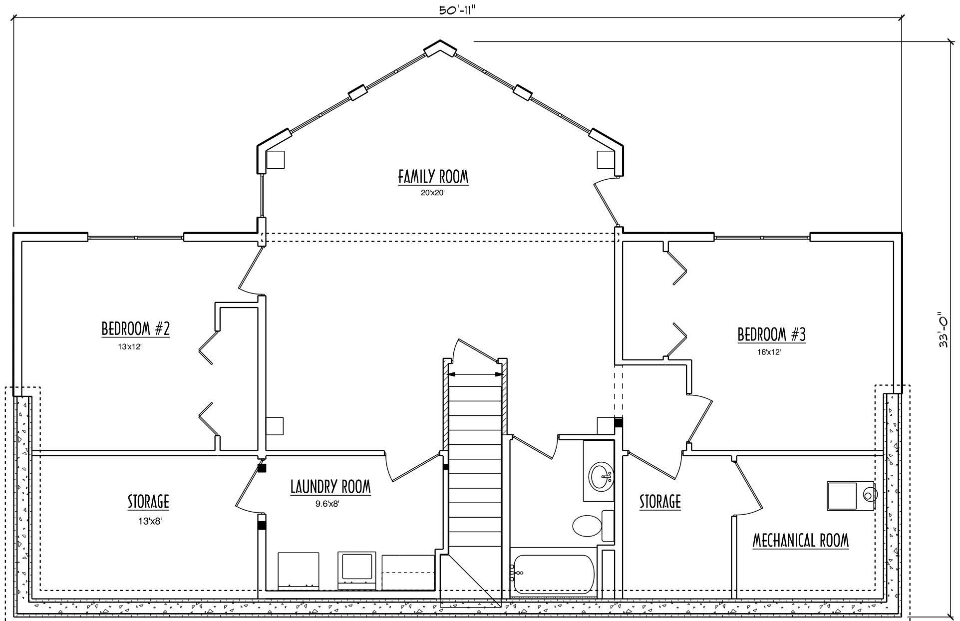
LOWER FLOOR PLAN 1253 Sq. Ft.
