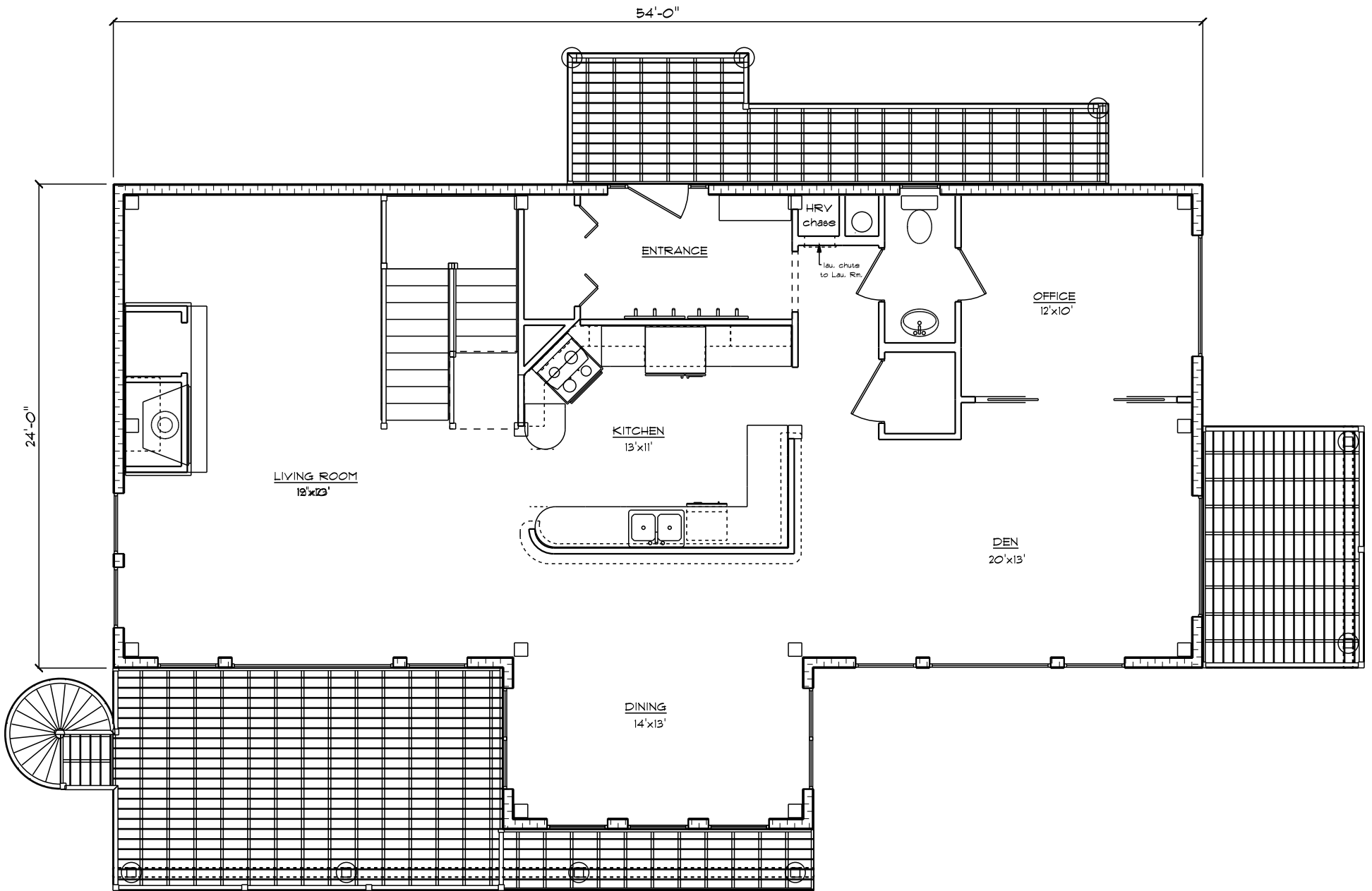
MAIN FLOOR PLAN Living - 1420 Sq. Ft.
